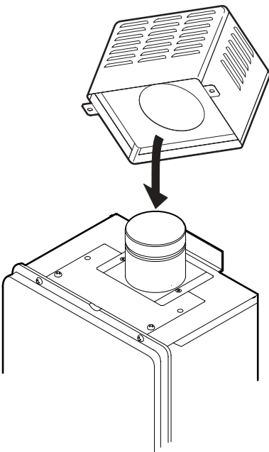
Figure 2a: Slide vent cap over flue.
