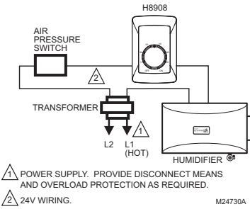
Fig. 15. Wiring H8908 in line with air pressure switch and humidifier.
