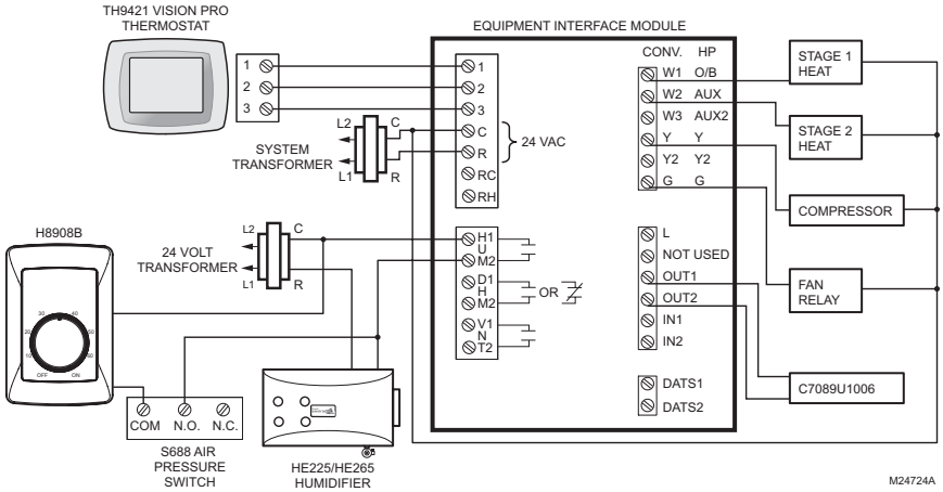
Fig. 17. Wiring H8908 with VisionPRO® IAQ on typical 2-stage furnace.
