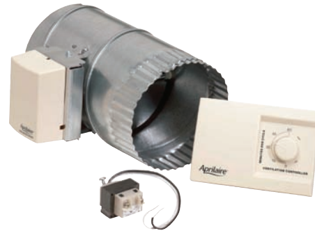
Model 8126 Ventilation Control System
