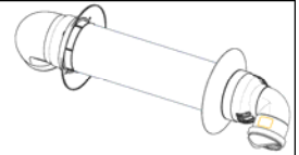
21" Non-Condensing Horizontal Termination Diverter Kit Part No.: 223187
