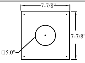
Metal Pass Through Plate Part No.: 224097
