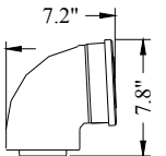
90 Degree Elbow (Metal) Part No.: 224255
