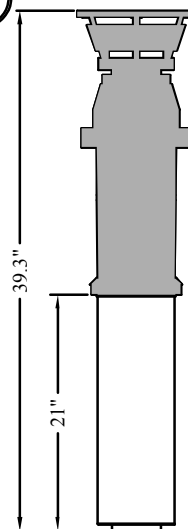
Roof Discharge Termination 18" Part No.: 184118-S
