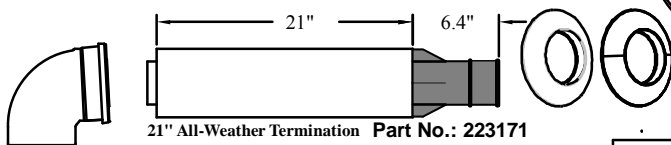
21" All-Weather Termination Part No.: 223171
