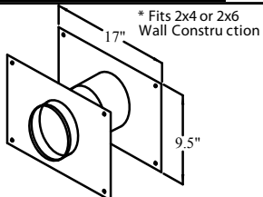
Thimble Part No.: 224045
