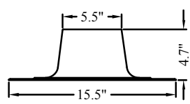
Roof Flashing - Flat Part No.: 146141
