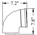
90 Degree Elbow (Metal) Part No.: 224255
