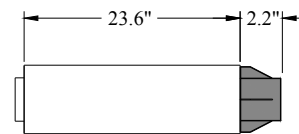
23.6" Standard Horizontal Termination (Metal) Part No.: 223155
