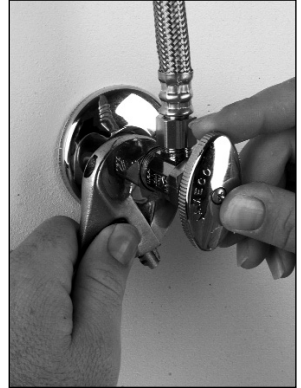
1. Turn off water supply and remove angle stops.
